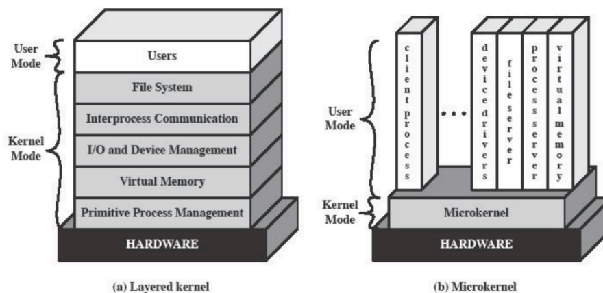
Figure 4.10 Kernel Architecture
